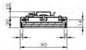
Rail Mount
