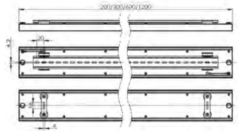
90mm Width
