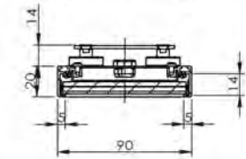
Magnetic Mount
